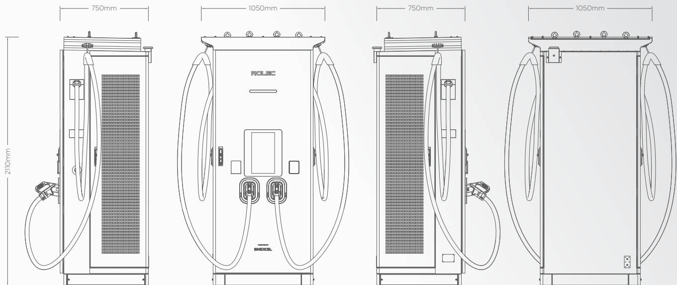
UltraCharge 240 with Cable Management System (CMS):
