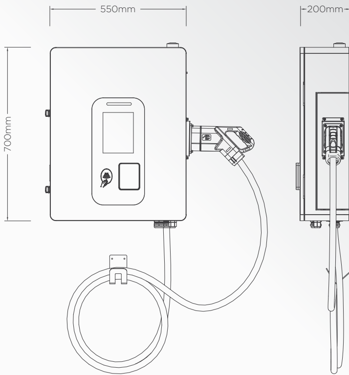
UltraCharge 30:
