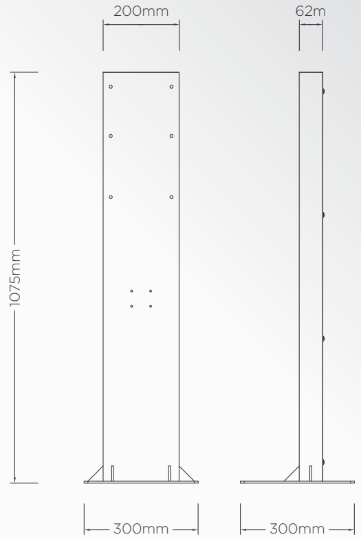
UltraCharge 30 Pedestal:
