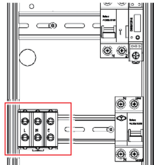
Figure 16 Incoming Mains Power Terminals (Single Phase Shown)
