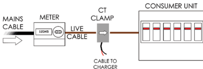
Figure 17 CT Clamp Positioning
