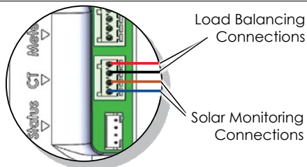
Figure 19 CT Connections for Load Balancing and Solar Monitoring
