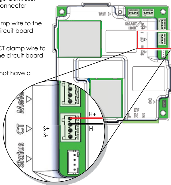
Figure 18 Load Balancing CT Connection
