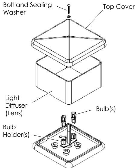
Figure 20 Lighting Head
