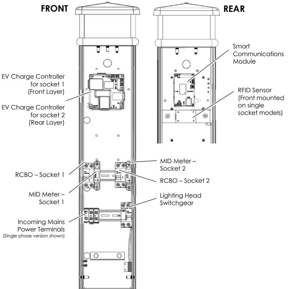
Figure 3 Internal Components - Typical Locations
