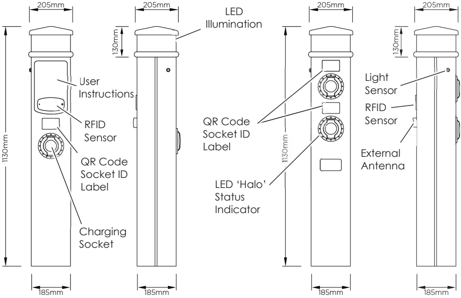
Figure 1 General Arrangement and Dimensions (Single and Double Socket Models)
