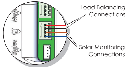
Figure 15 CT Connections for Load Balancing and Solar Monitoring
