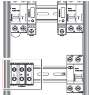
Figure 12 Incoming Mains Power Terminals (Single Phase Shown)
