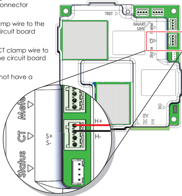
Figure 14 Load Balancing CT Connection
