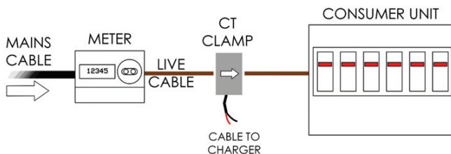
Figure 13 CT Clamp Positioning
