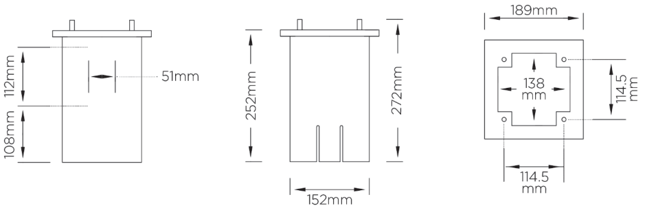
Figure 2 Optional Ground Mounting Base
