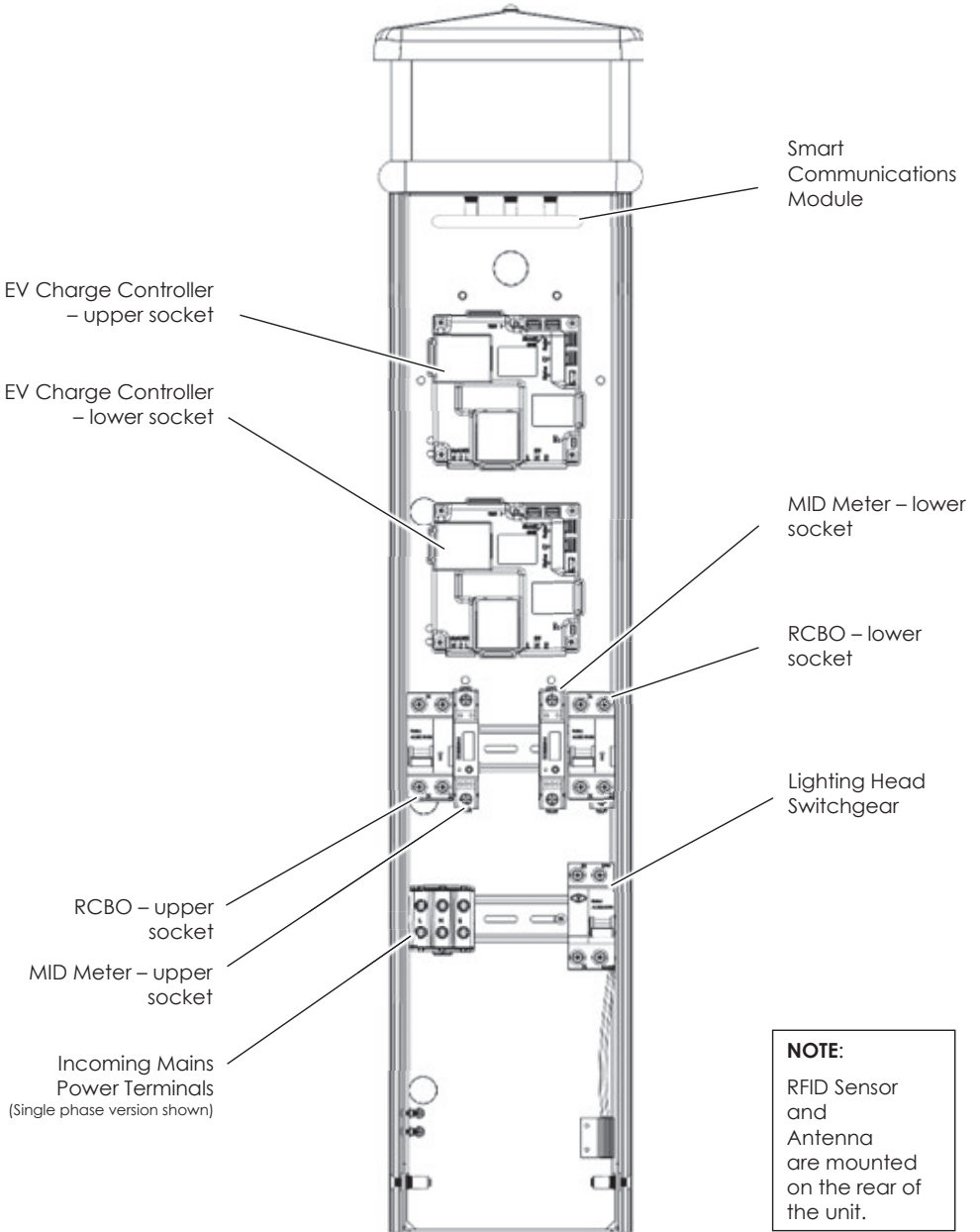
Figure 3 Internal Components - Typical Locations
